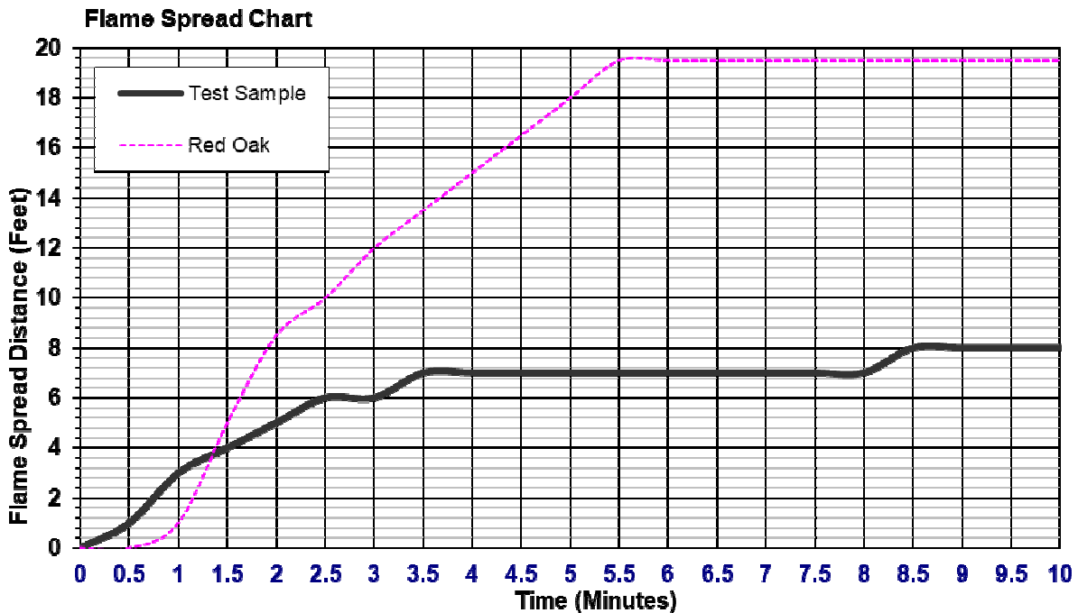
Figure 1 Flame Spread Chart
